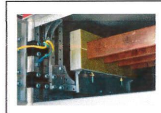
母线夹
